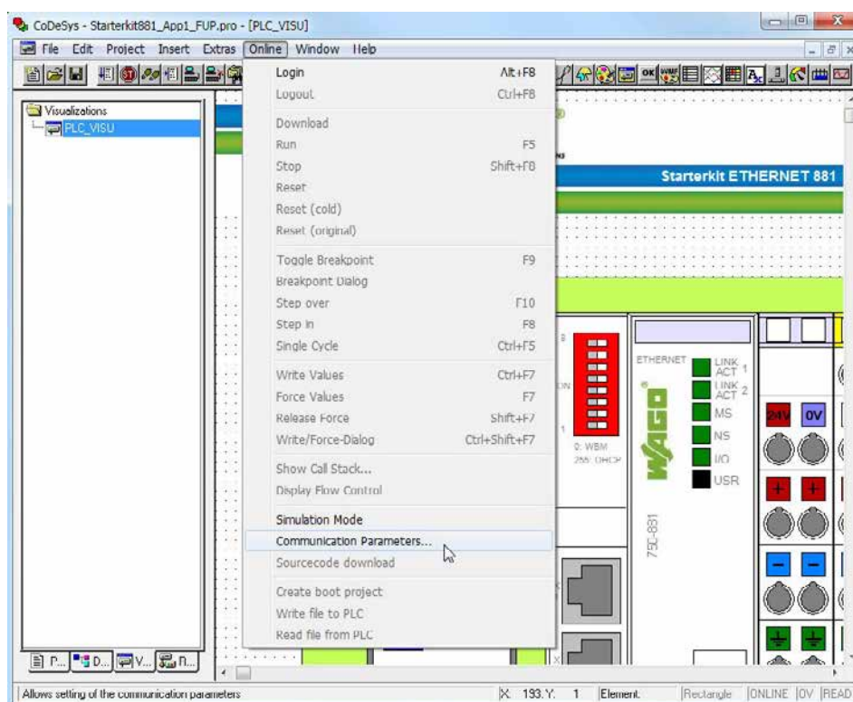
Figure 43: Communication parameters
