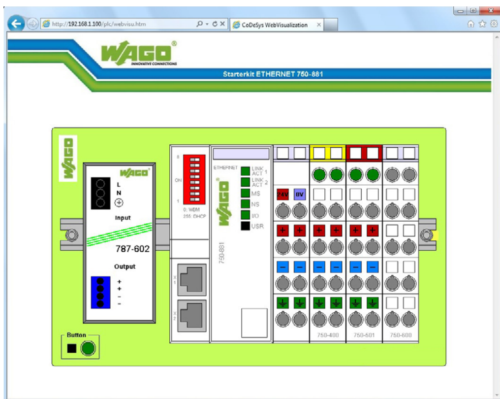
Figure 24: Web visualization
