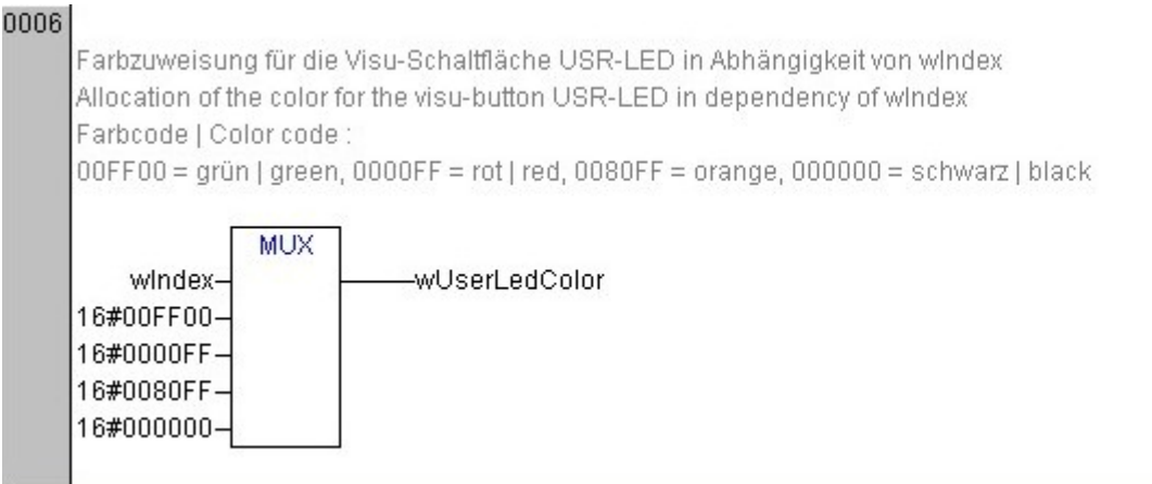
Figure 42: Network 6 (USR-LED)
