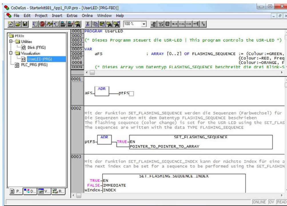
Figure 36: "UserLED" program
