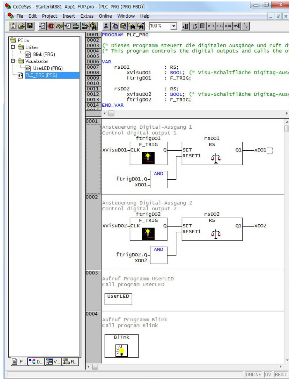
Figure 30: "PLC_PRG" program
