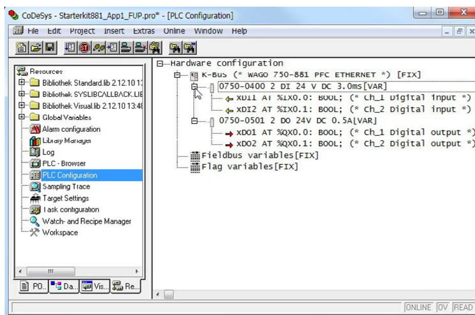
Figure 25: PLC configuration
